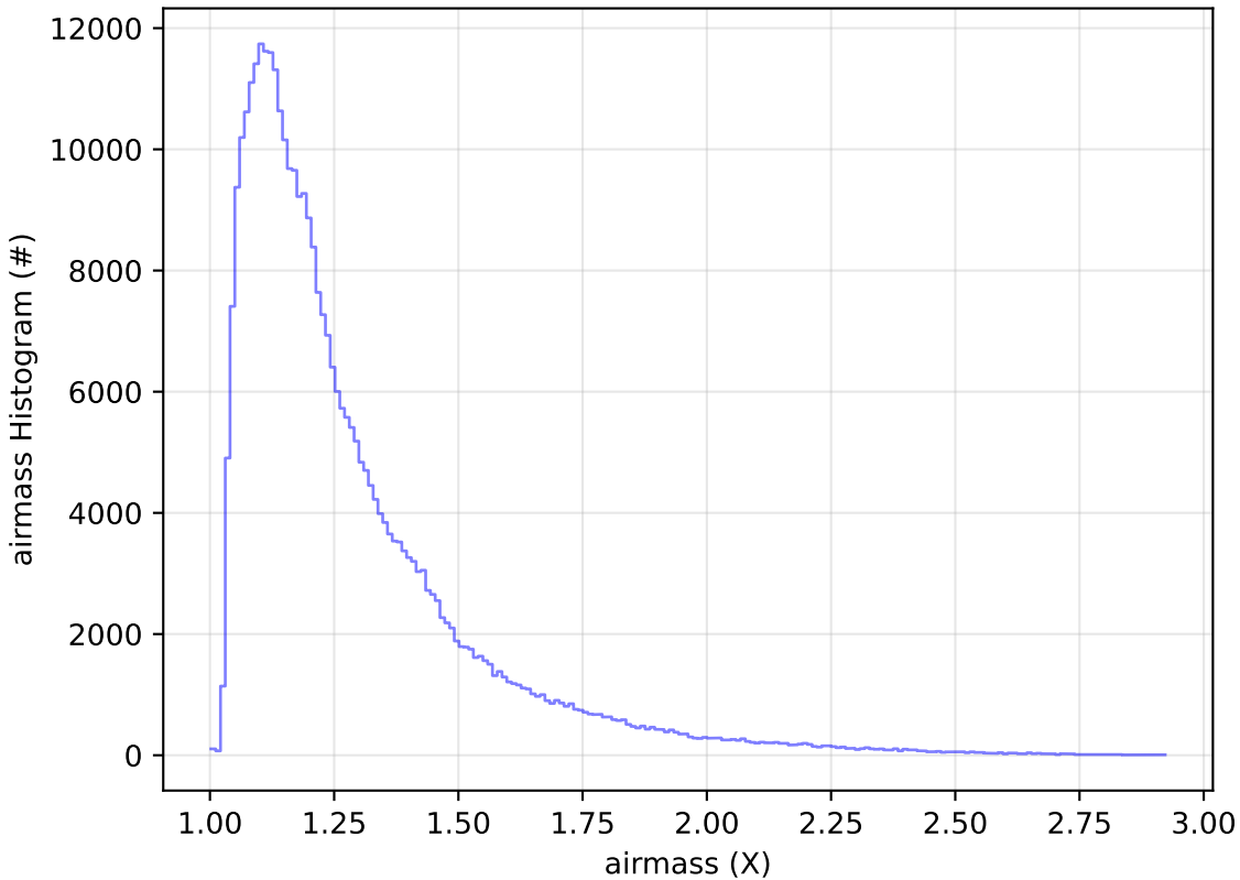
baseline_v3.5_10yrs WFD y band: airmass Histogram
