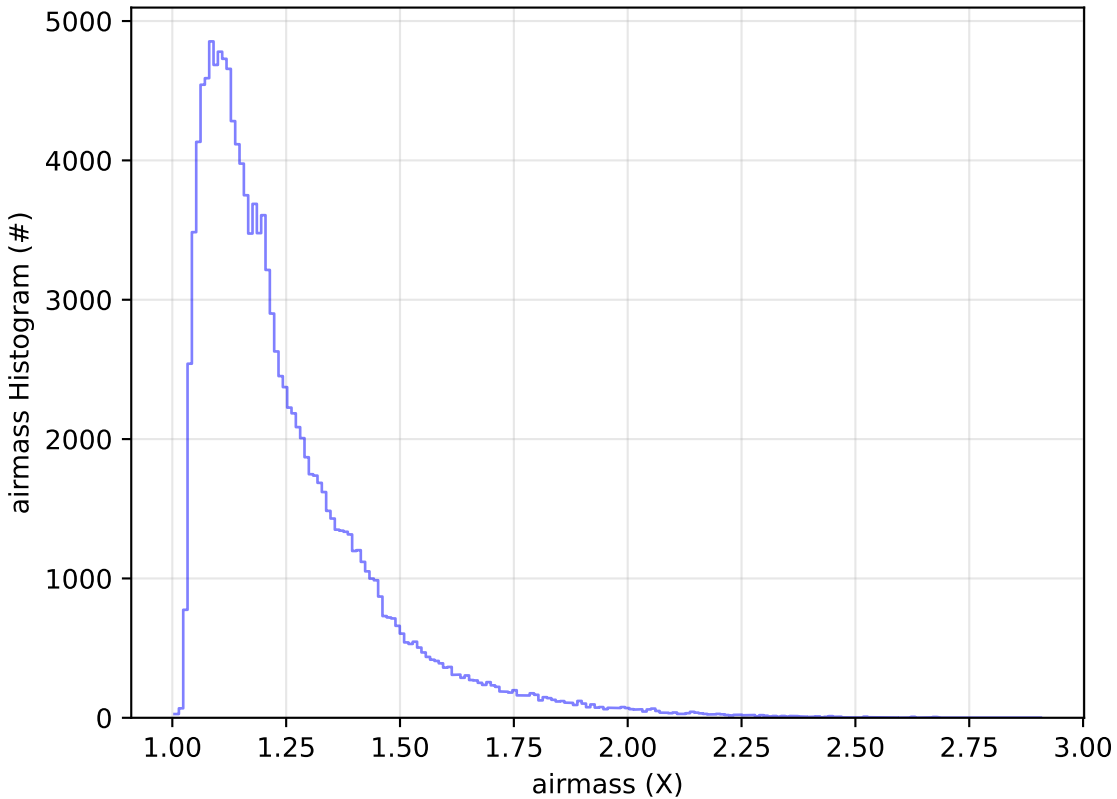
baseline_v3.5_10yrs WFD u band: airmass Histogram
