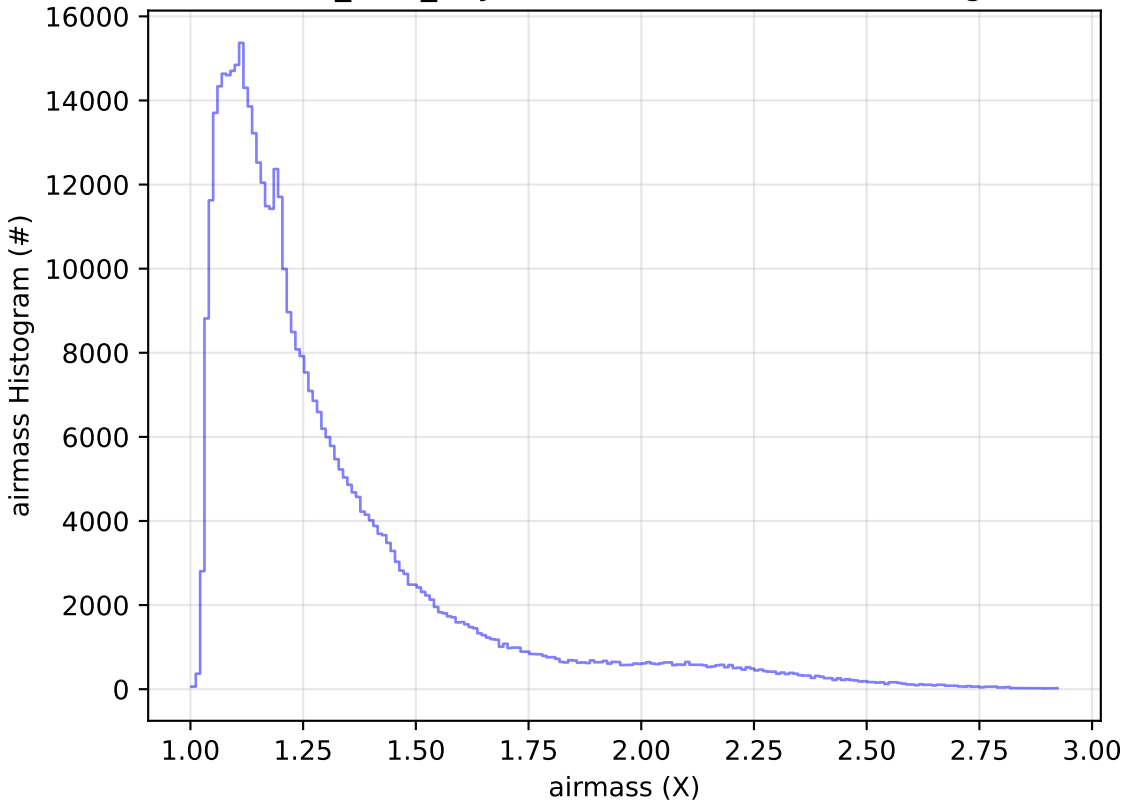
baseline_v3.5_10yrs WFD r band: airmass Histogram
