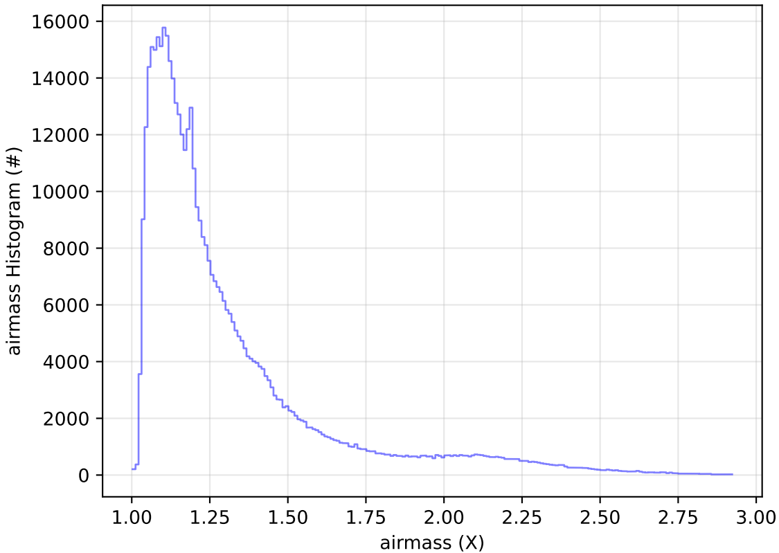
baseline_v3.5_10yrs WFD i band: airmass Histogram
