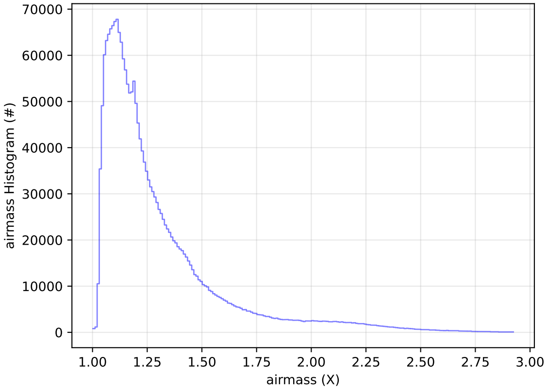
baseline_v3.5_10yrs WFD all bands: airmass Histogram
