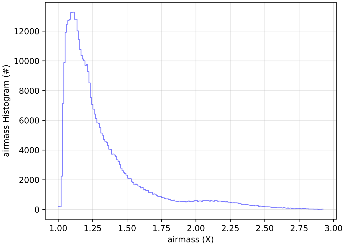
baseline_v3.5_10yrs All sky z band: airmass Histogram
