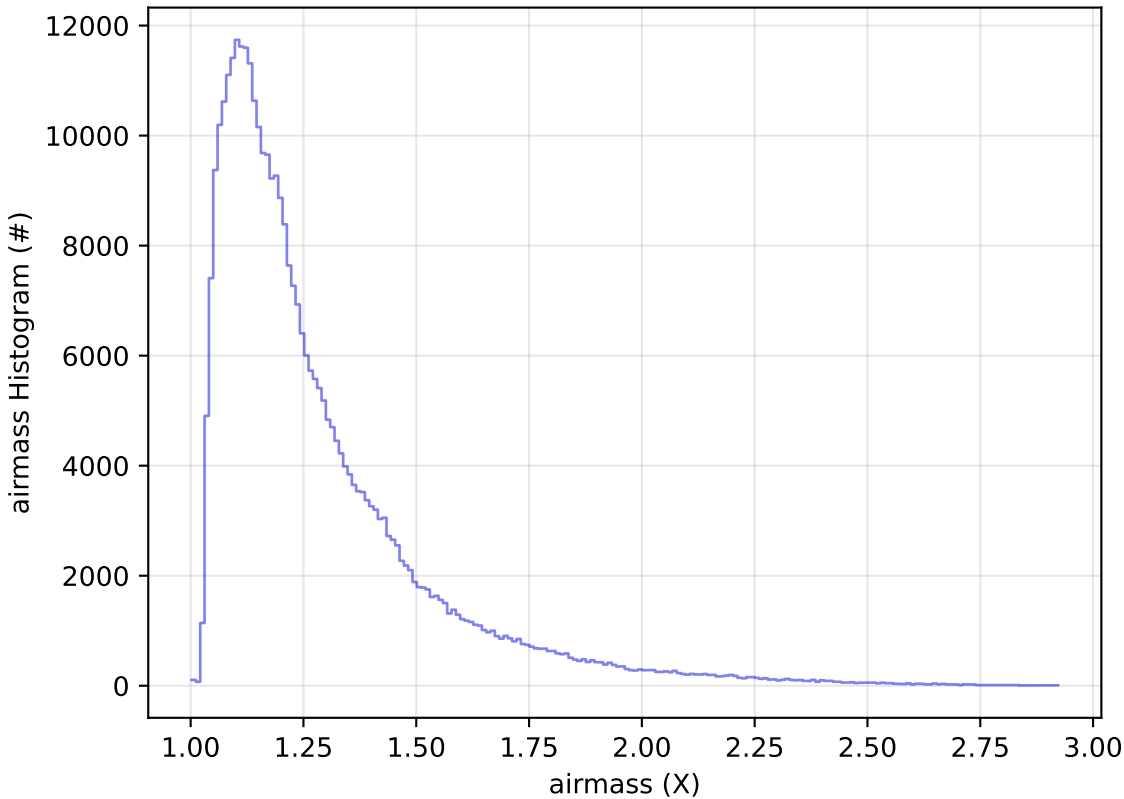
baseline_v3.5_10yrs All sky y band: airmass Histogram
