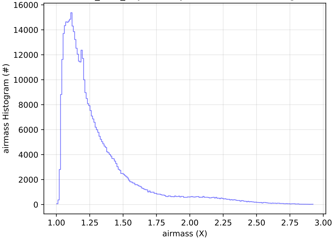
baseline_v3.5_10yrs All sky r band: airmass Histogram
