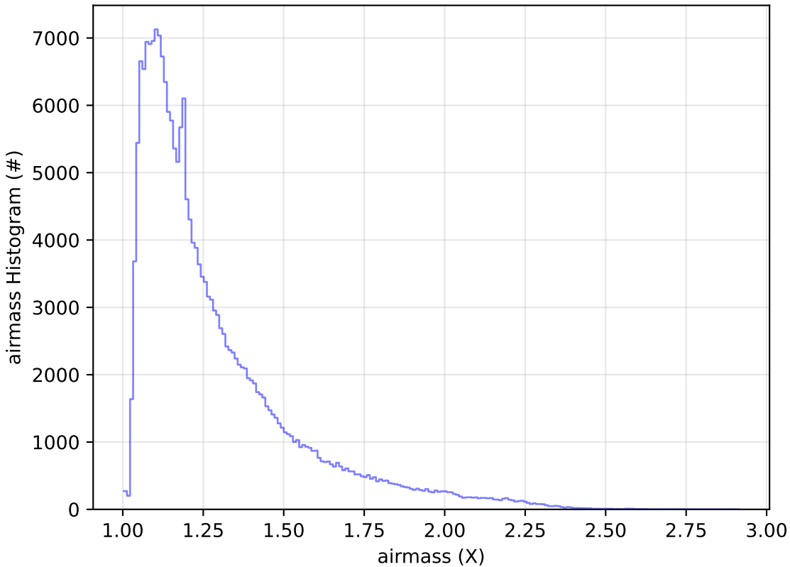
baseline_v3.5_10yrs All sky g band: airmass Histogram
