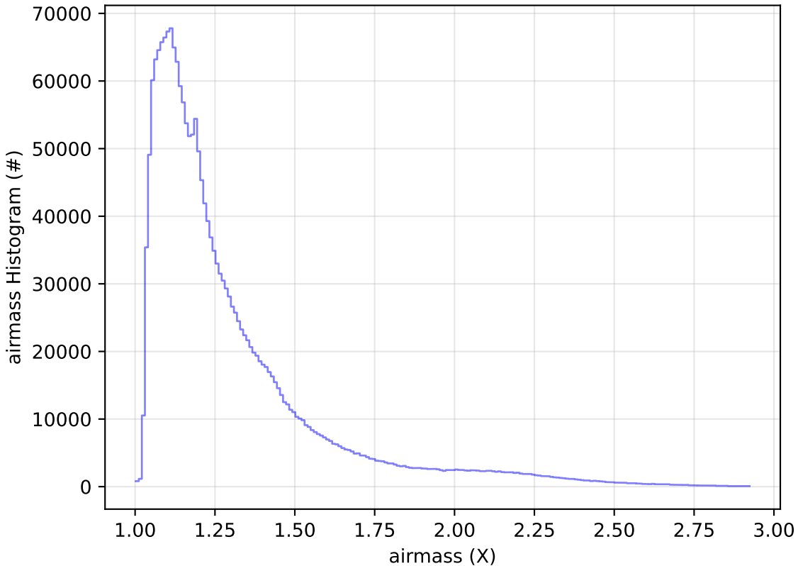
baseline_v3.5_10yrs All sky all bands: airmass Histogram
