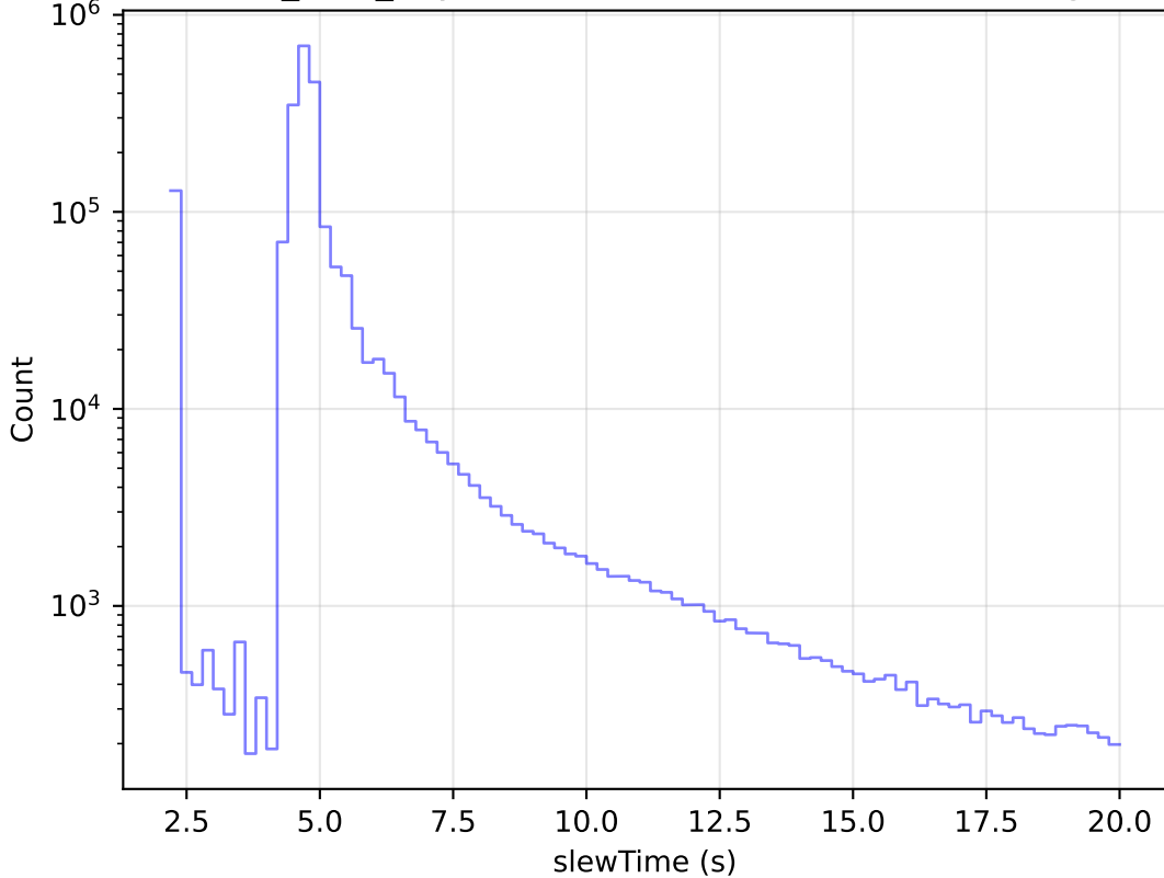
baseline_v3.5_10yrs All visits: Zoom Slew Time Histogram
