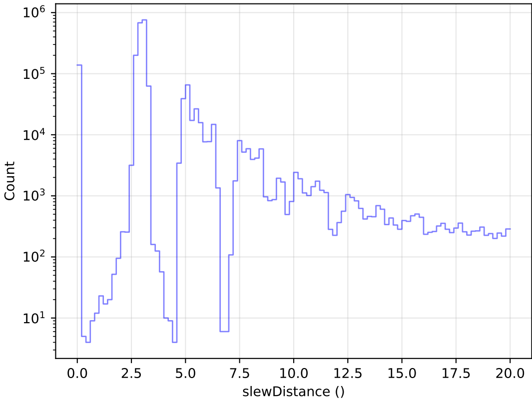
baseline_v3.5_10yrs All visits: Zoom Slew Distance Histogram
