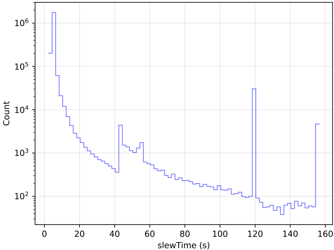
baseline_v3.5_10yrs All visits: Slew Time Histogram
