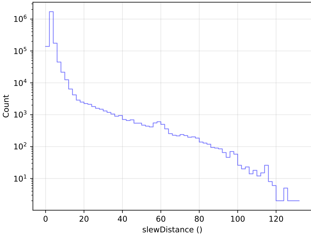
baseline_v3.5_10yrs All visits: Slew Distance Histogram
