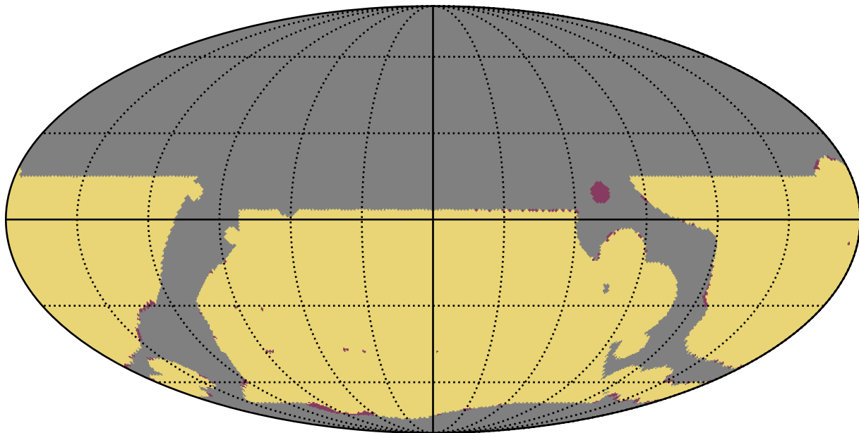
baseline_v3.5_10yrs WFD: RapidRevisits
