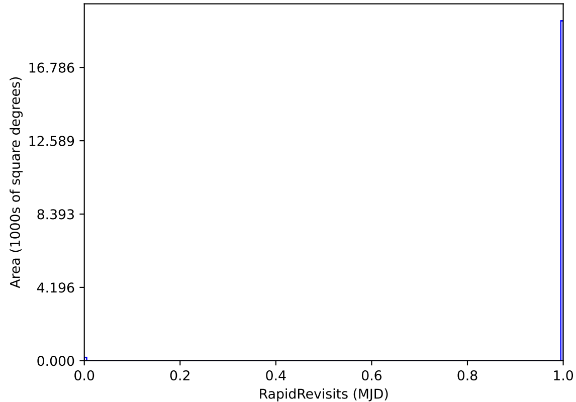
baseline_v3.5_10yrs WFD: RapidRevisits
