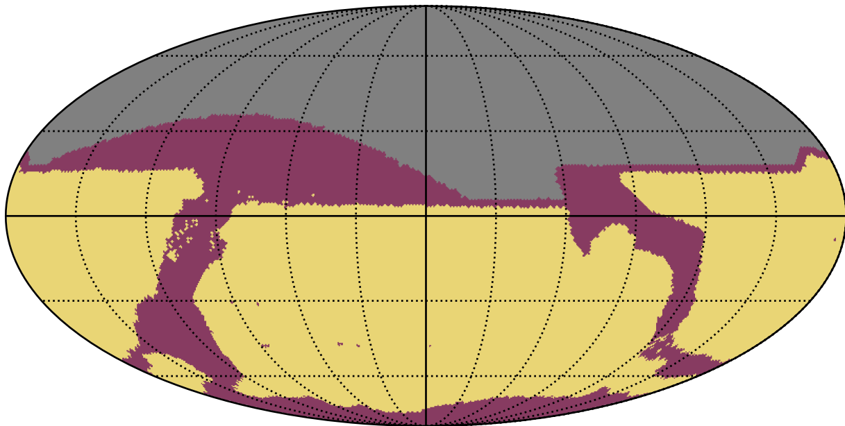
baseline_v3.5_10yrs All sky: RapidRevisits
