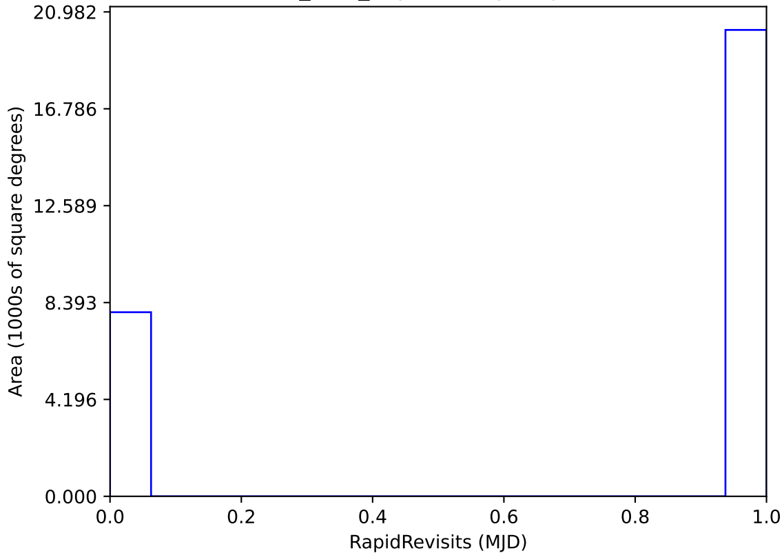
baseline_v3.5_10yrs All sky: RapidRevisits
