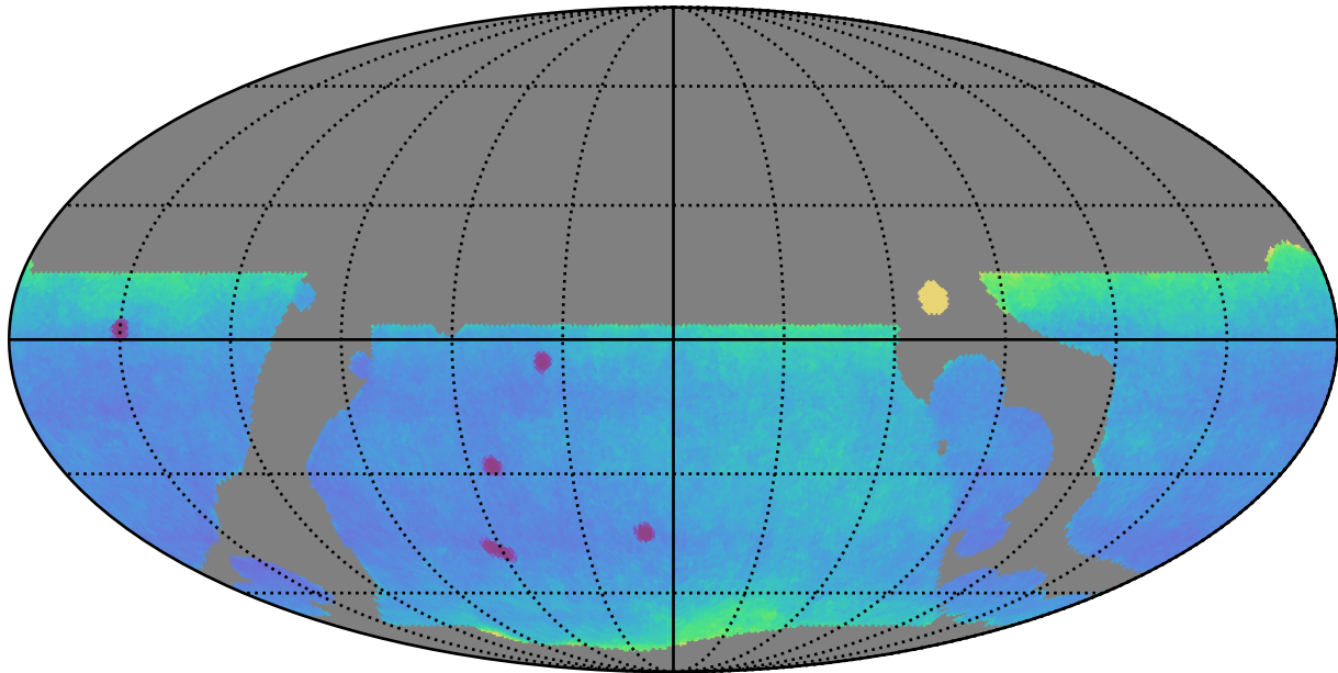
baseline_v3.5_10yrs WFD: Proper Motion Uncert @ 24.0
