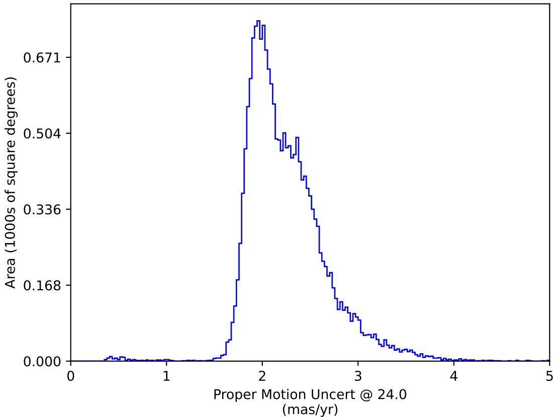
baseline_v3.5_10yrs WFD: Proper Motion Uncert @ 24.0
