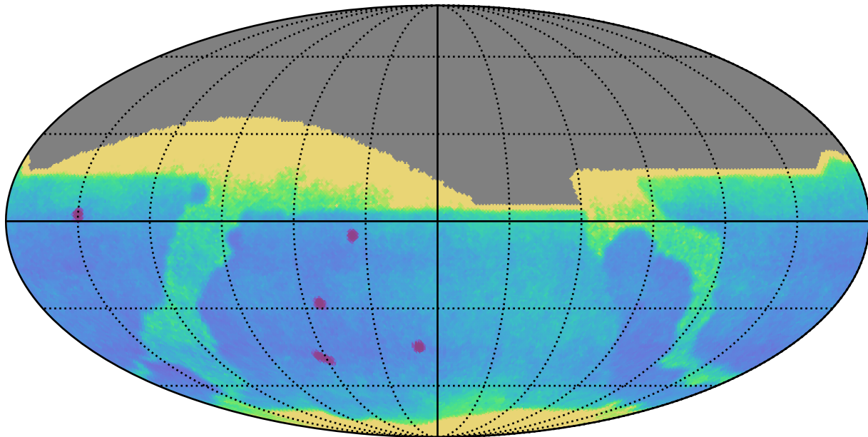
baseline_v3.5_10yrs All sky: Proper Motion Uncert @ 24.0
