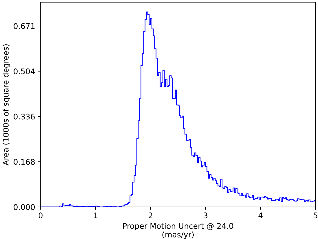
baseline_v3.5_10yrs All sky: Proper Motion Uncert @ 24.0
