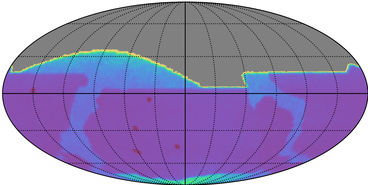
baseline_v3.5_10yrs All sky: Proper Motion Uncert @ 20.5
