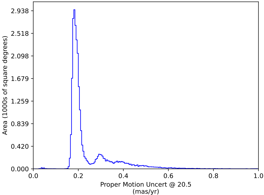
baseline_v3.5_10yrs All sky: Proper Motion Uncert @ 20.5
