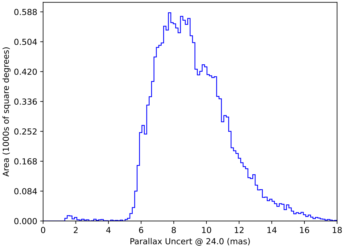
baseline_v3.5_10yrs WFD: Parallax Uncert @ 24.0
