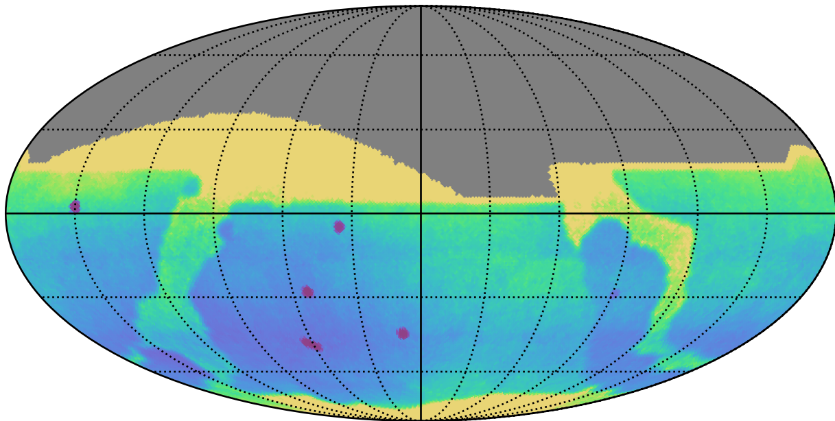
baseline_v3.5_10yrs All sky: Parallax Uncert @ 24.0
