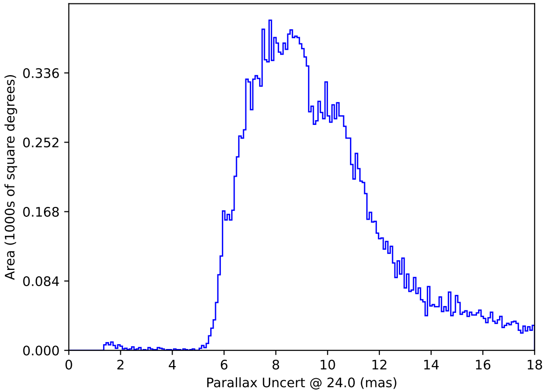
baseline_v3.5_10yrs All sky: Parallax Uncert @ 24.0
