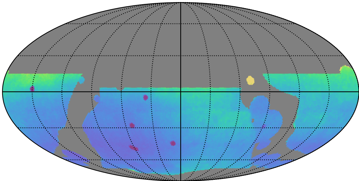
baseline_v3.5_10yrs WFD: Parallax Uncert @ 22.4
