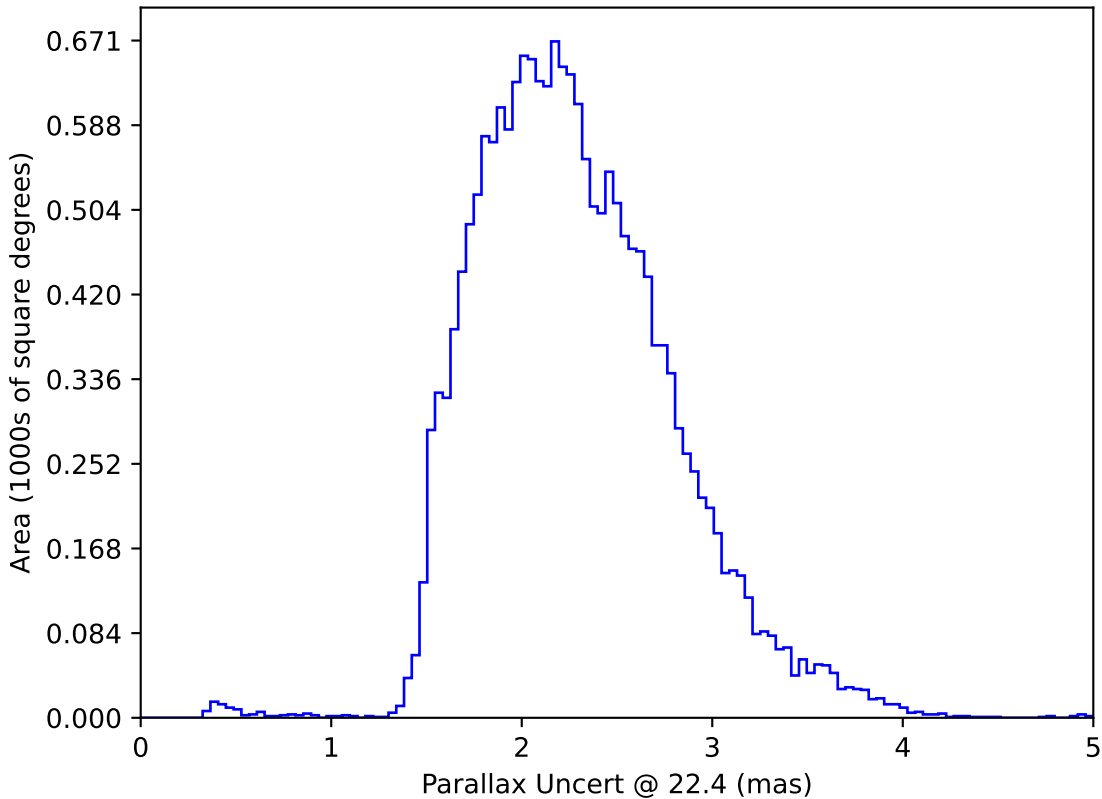
baseline_v3.5_10yrs WFD: Parallax Uncert @ 22.4
