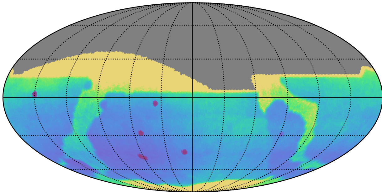
baseline_v3.5_10yrs All sky: Parallax Uncert @ 22.4
