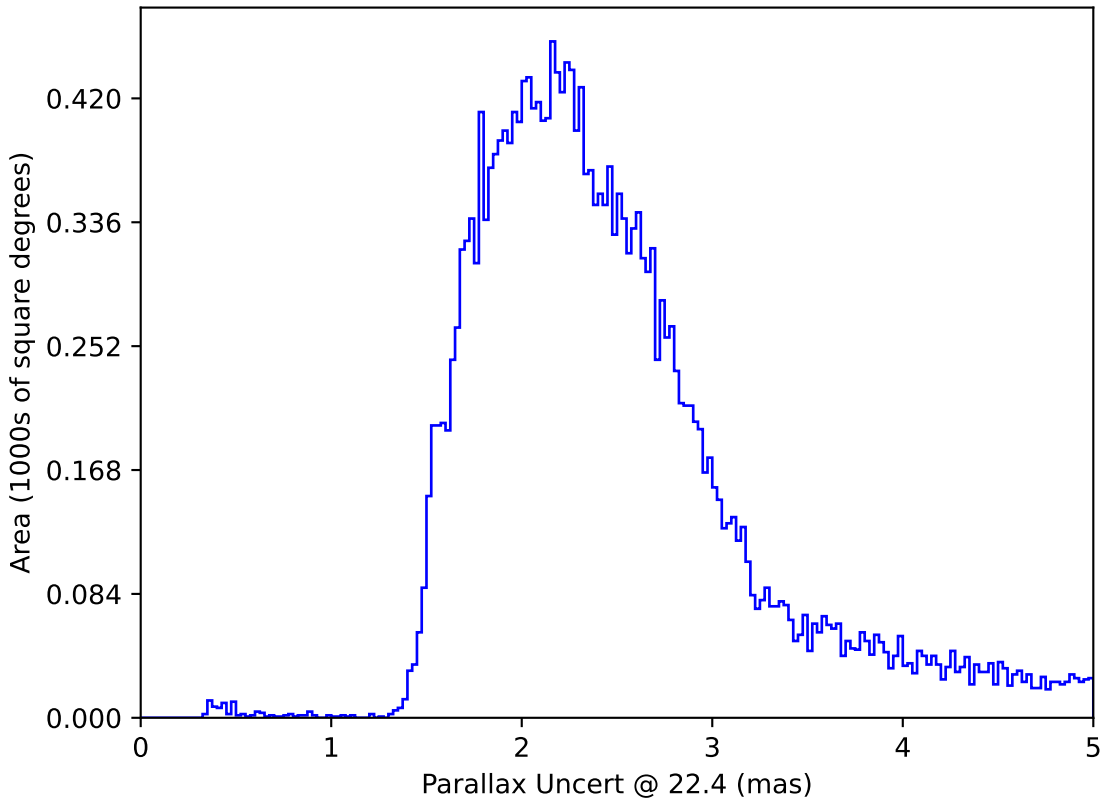
baseline_v3.5_10yrs All sky: Parallax Uncert @ 22.4
