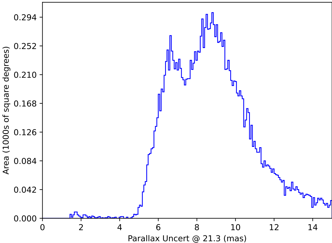
baseline_v3.5_10yrs WFD y band only: Parallax Uncert @ 21.3
