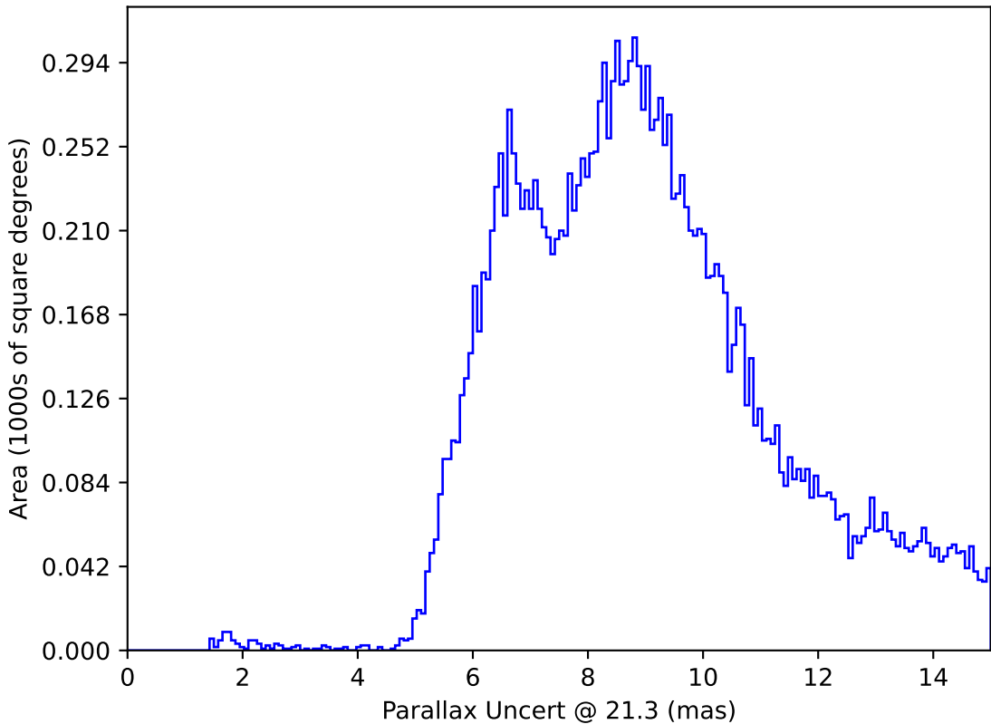
baseline_v3.5_10yrs All sky y band only: Parallax Uncert @ 21.3
