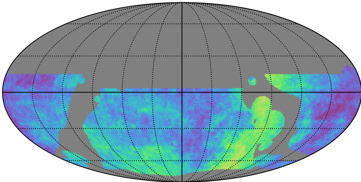
baseline_v3.5_10yrs WFD: Parallax Coverage @ 24.0
