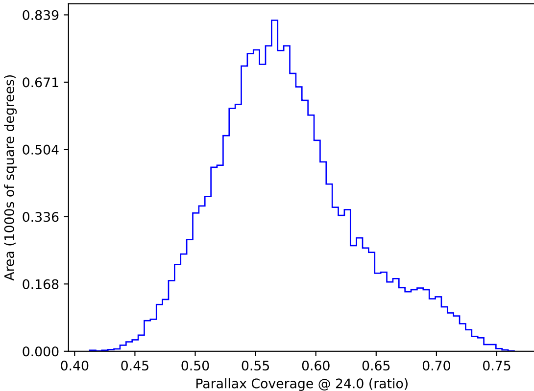
baseline_v3.5_10yrs WFD: Parallax Coverage @ 24.0
