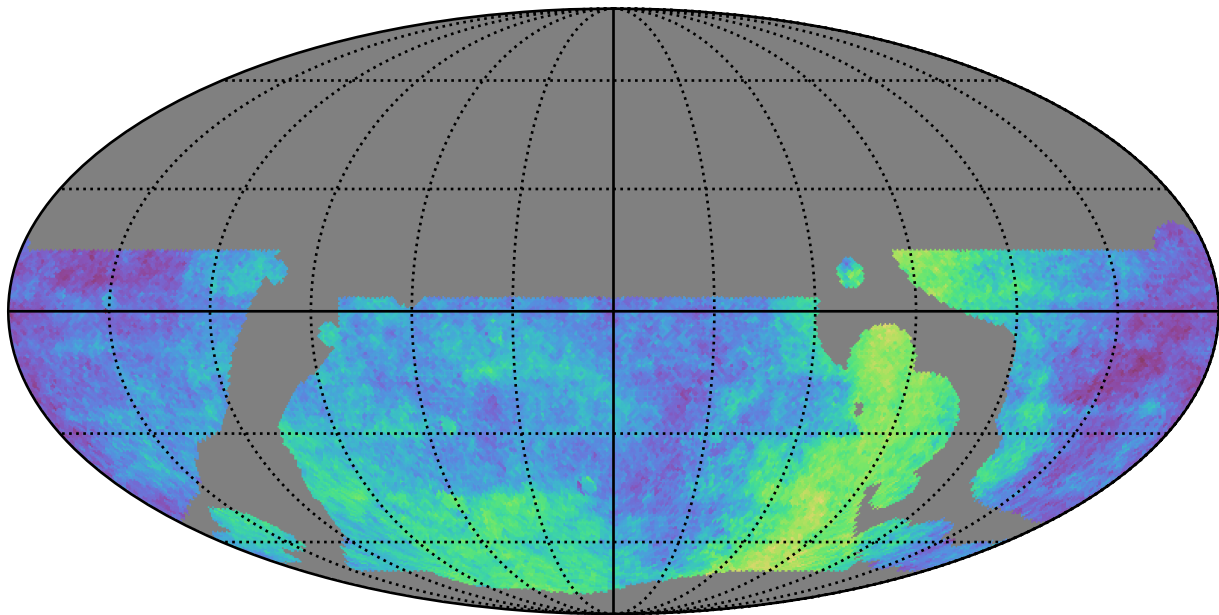
baseline_v3.5_10yrs WFD: Parallax Coverage @ 22.4
