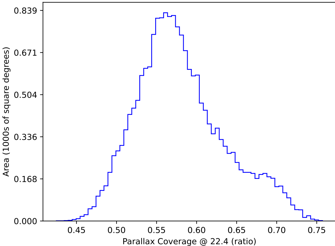
baseline_v3.5_10yrs WFD: Parallax Coverage @ 22.4
