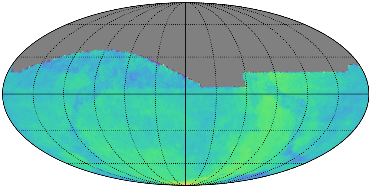
baseline_v3.5_10yrs All sky: Parallax Coverage @ 22.4
