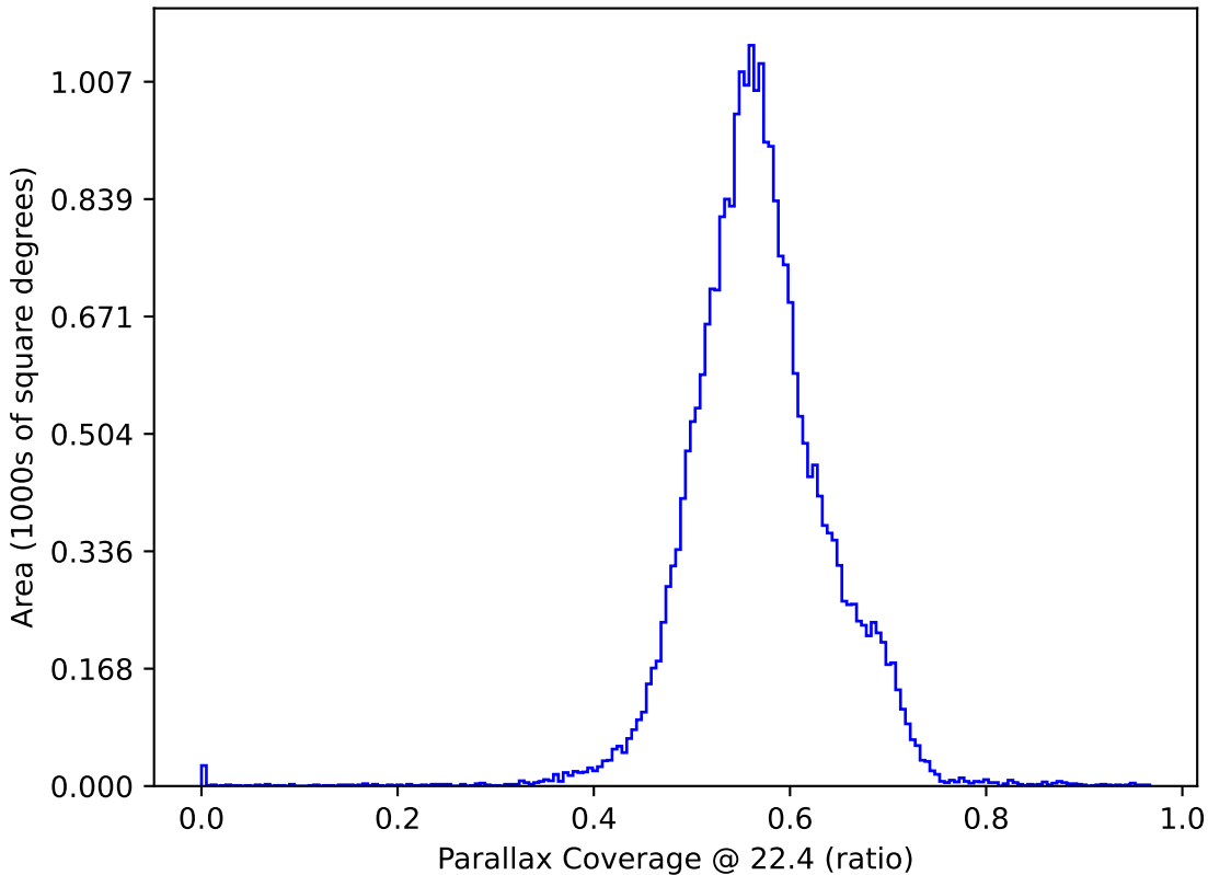
baseline_v3.5_10yrs All sky: Parallax Coverage @ 22.4
