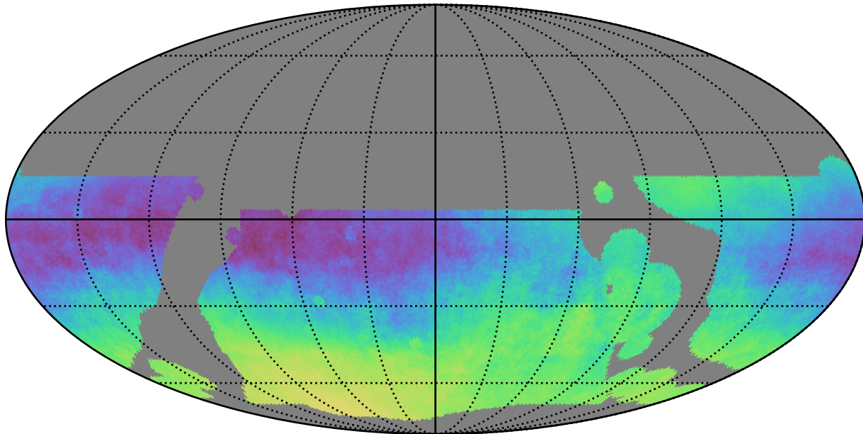
baseline_v3.5_10yrs WFD: Parallax-DCR degeneracy @ 24.0
