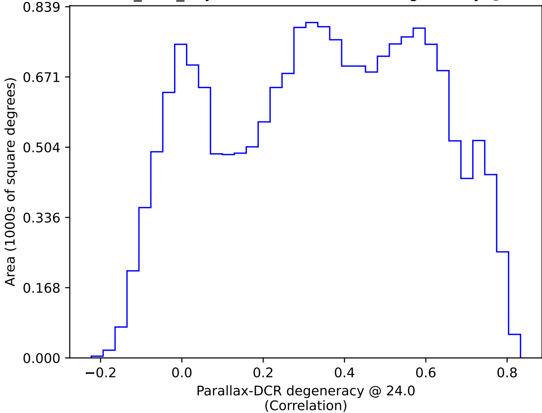
baseline_v3.5_10yrs WFD: Parallax-DCR degeneracy @ 24.0
