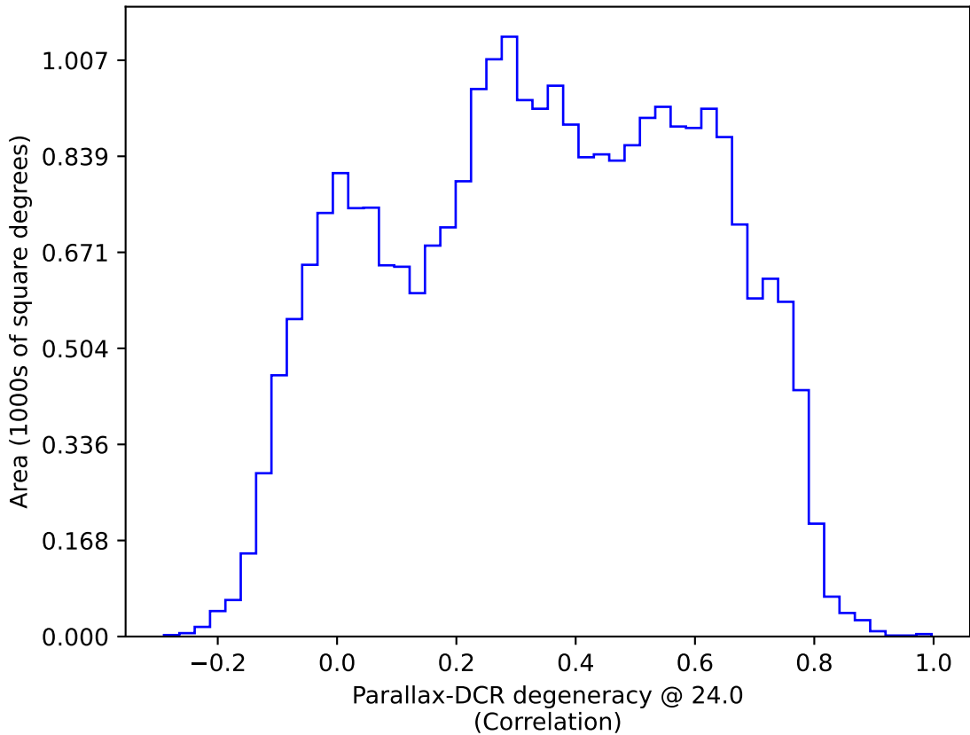
baseline_v3.5_10yrs All sky: Parallax-DCR degeneracy @ 24.0
