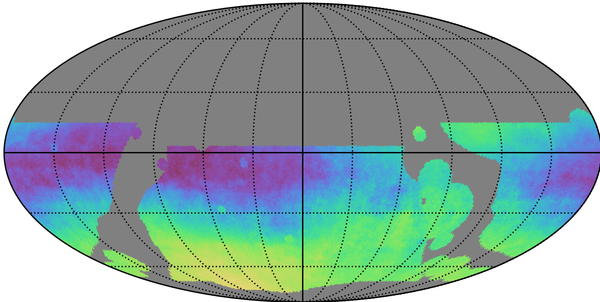
baseline_v3.5_10yrs WFD: Parallax-DCR degeneracy @ 22.4
