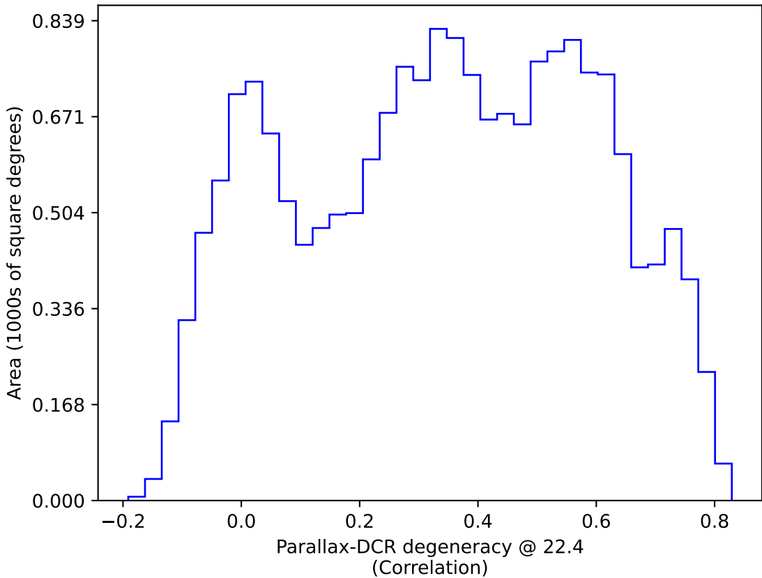
baseline_v3.5_10yrs WFD: Parallax-DCR degeneracy @ 22.4
