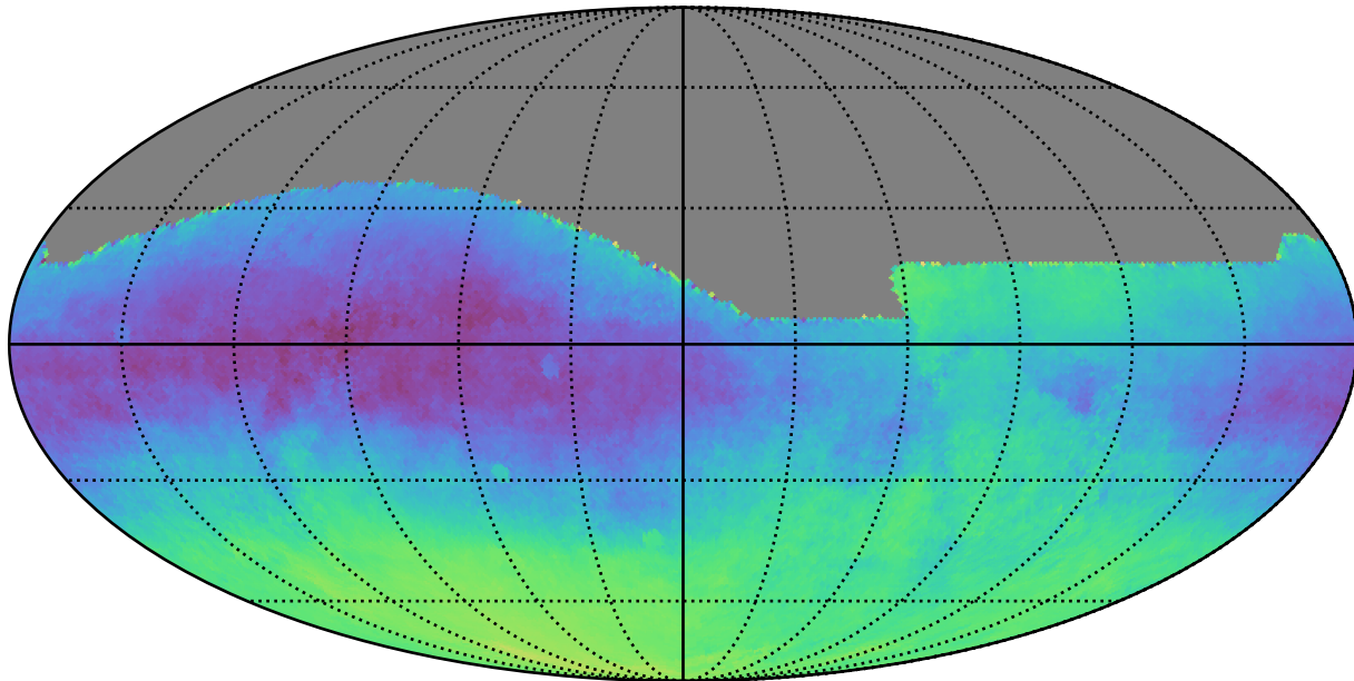
baseline_v3.5_10yrs All sky: Parallax-DCR degeneracy @ 22.4
