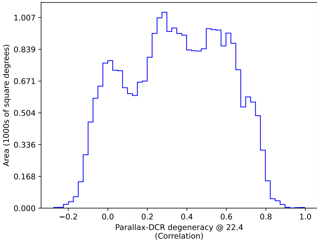
baseline_v3.5_10yrs All sky: Parallax-DCR degeneracy @ 22.4
