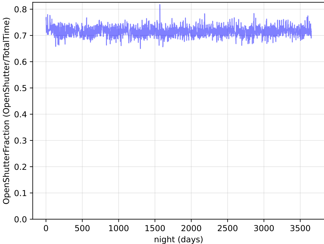
baseline_v3.5_10yrs Per night: OpenShutterFraction
