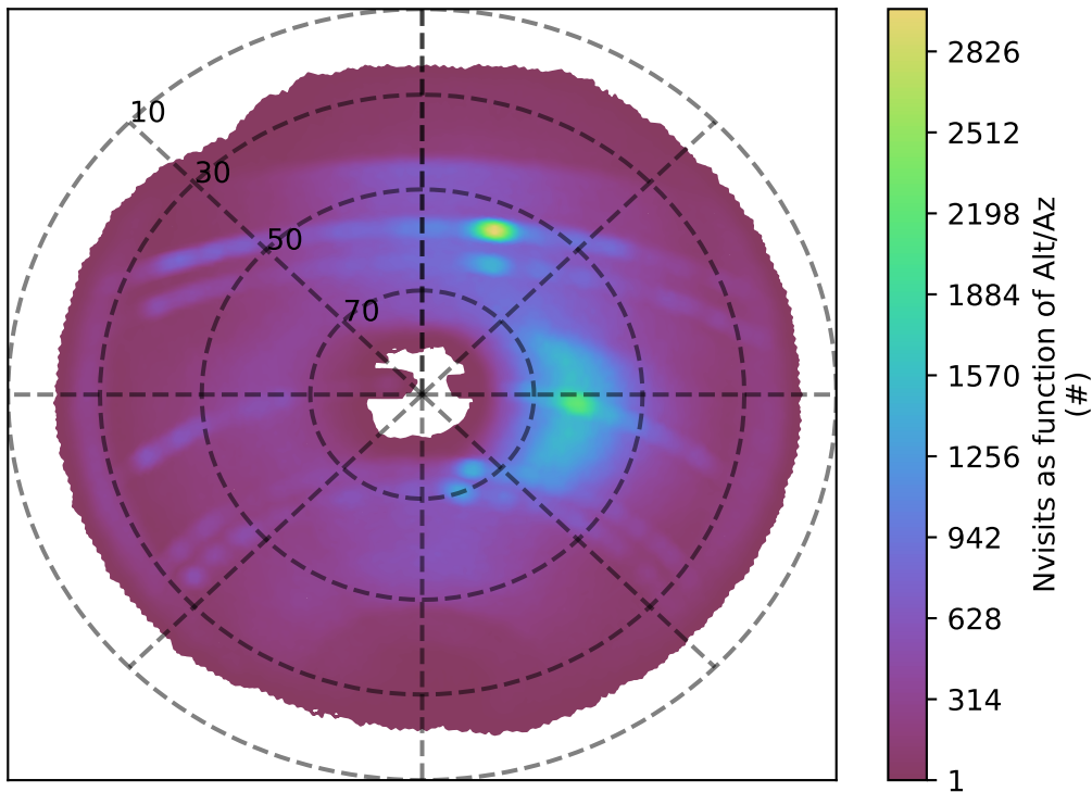
baseline_v3.5_10yrs z band: Nvisits as function of Alt/Az
