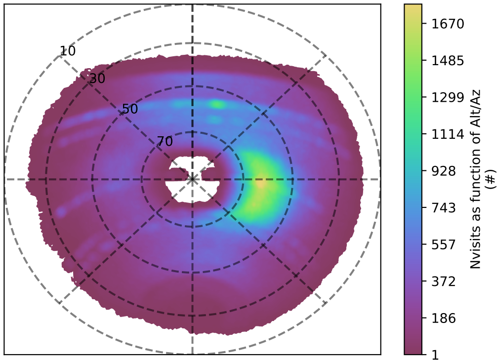
baseline_v3.5_10yrs y band: Nvisits as function of Alt/Az
