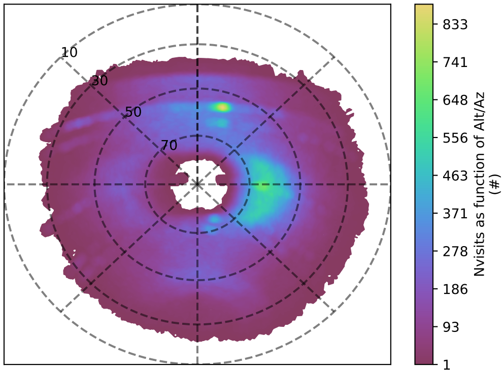
baseline_v3.5_10yrs u band: Nvisits as function of Alt/Az
